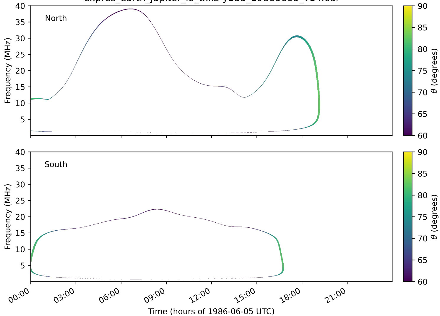
expres_earth_jupiter_io_txka-y235_19860605_v14.cdf
