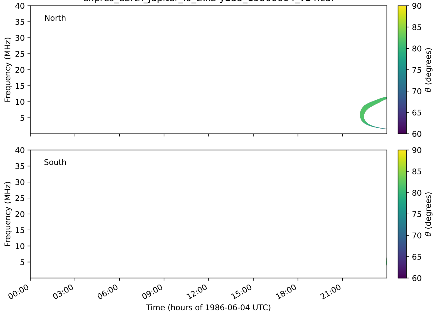
expres_earth_jupiter_io_txka-y235_19860604_v14.cdf
