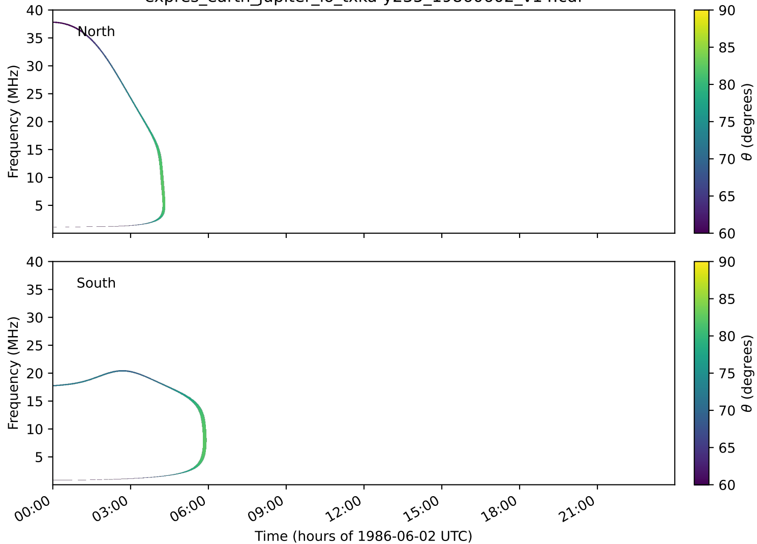
expres_earth_jupiter_io_txka-y235_19860602_v14.cdf
