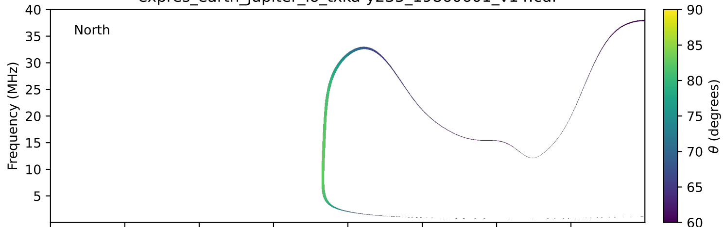
expres_earth_jupiter_io_txka-y235_19860601_v14.cdf
