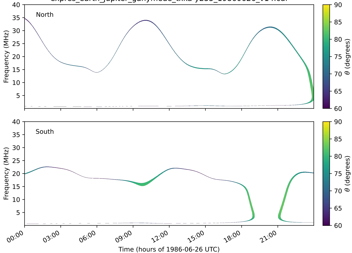
expres_earth_jupiter_ganymede_txka-y235_19860626_v14.cdf
