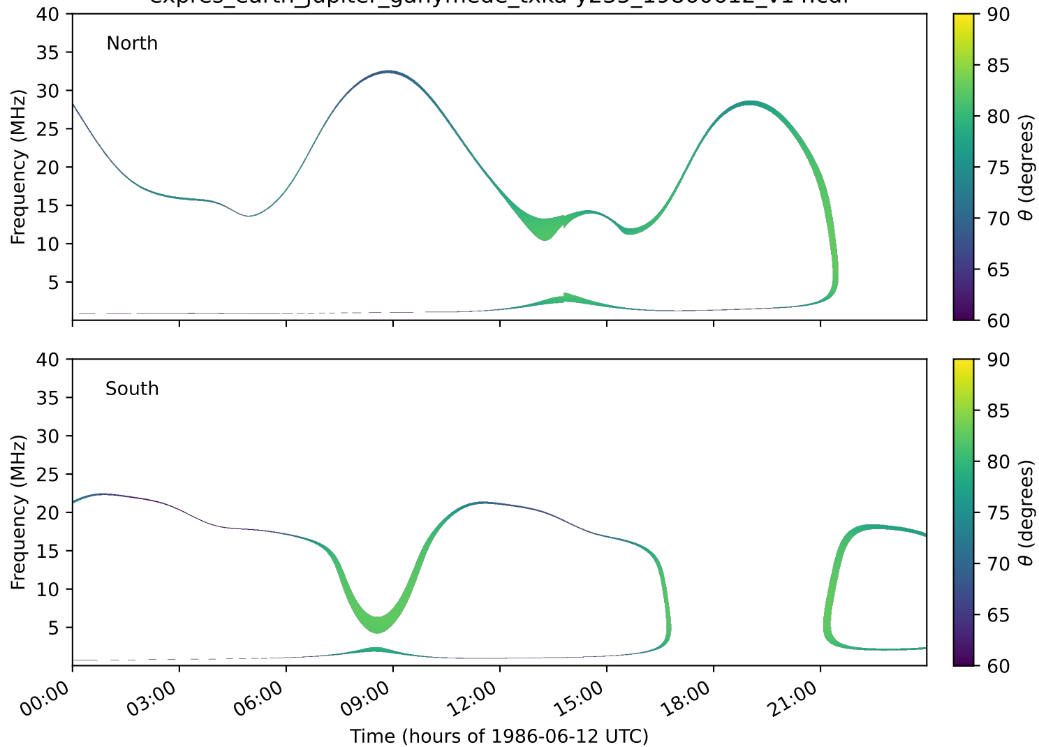
expres_earth_jupiter_ganymede_txka-y235_19860612_v14.cdf
