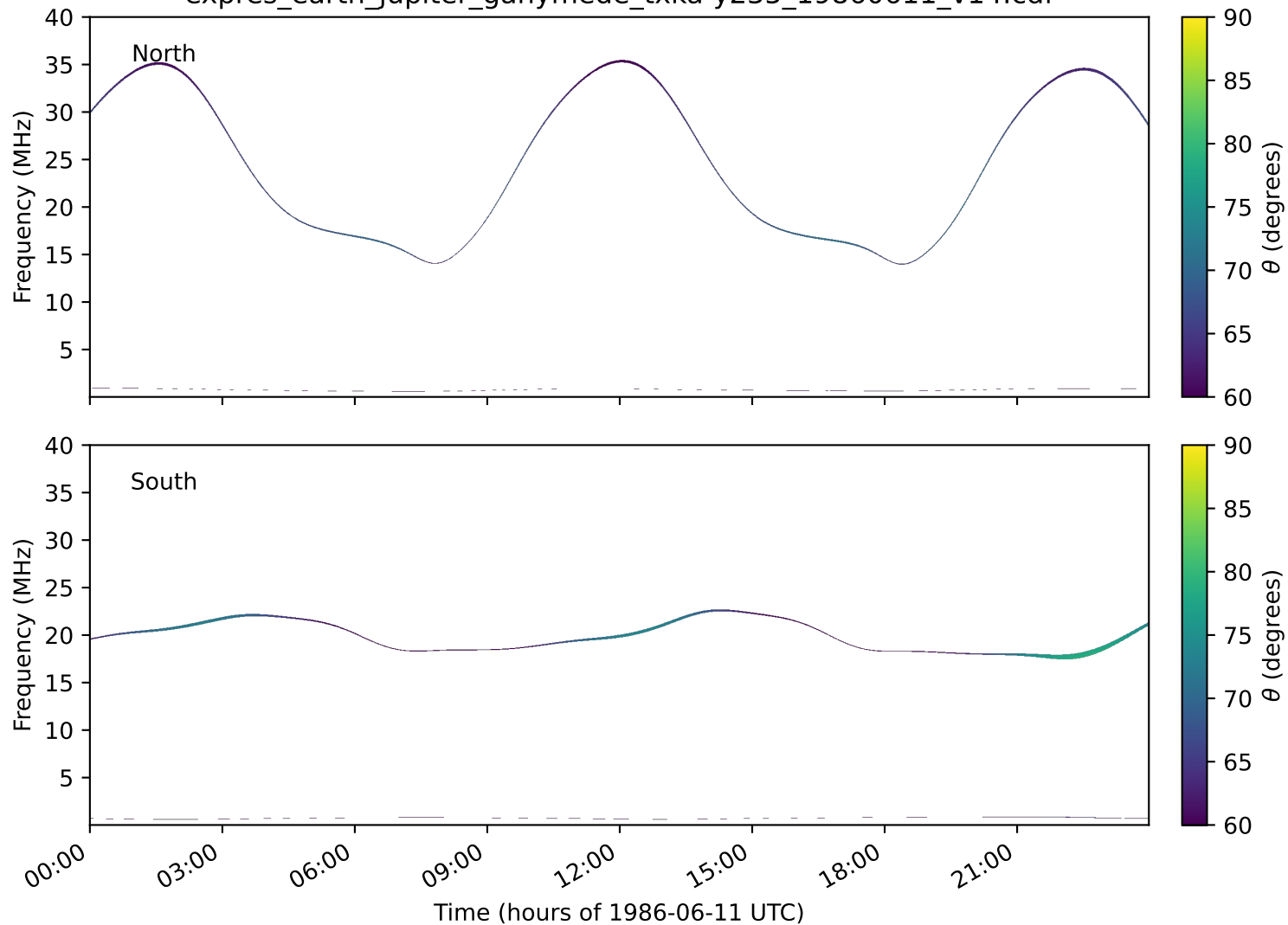
expres_earth_jupiter_ganymede_txka-y235_19860611_v14.cdf
