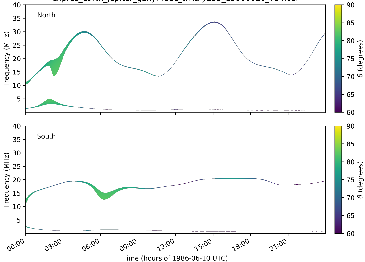
expres_earth_jupiter_ganymede_txka-y235_19860610_v14.cdf
