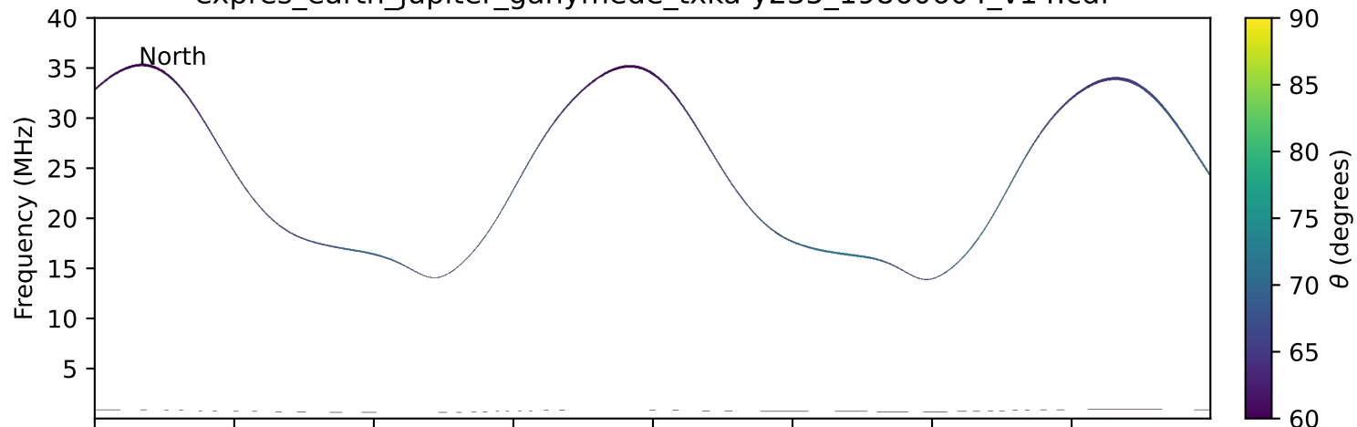
expres_earth_jupiter_ganymede_txka-y235_19860604_v14.cdf
