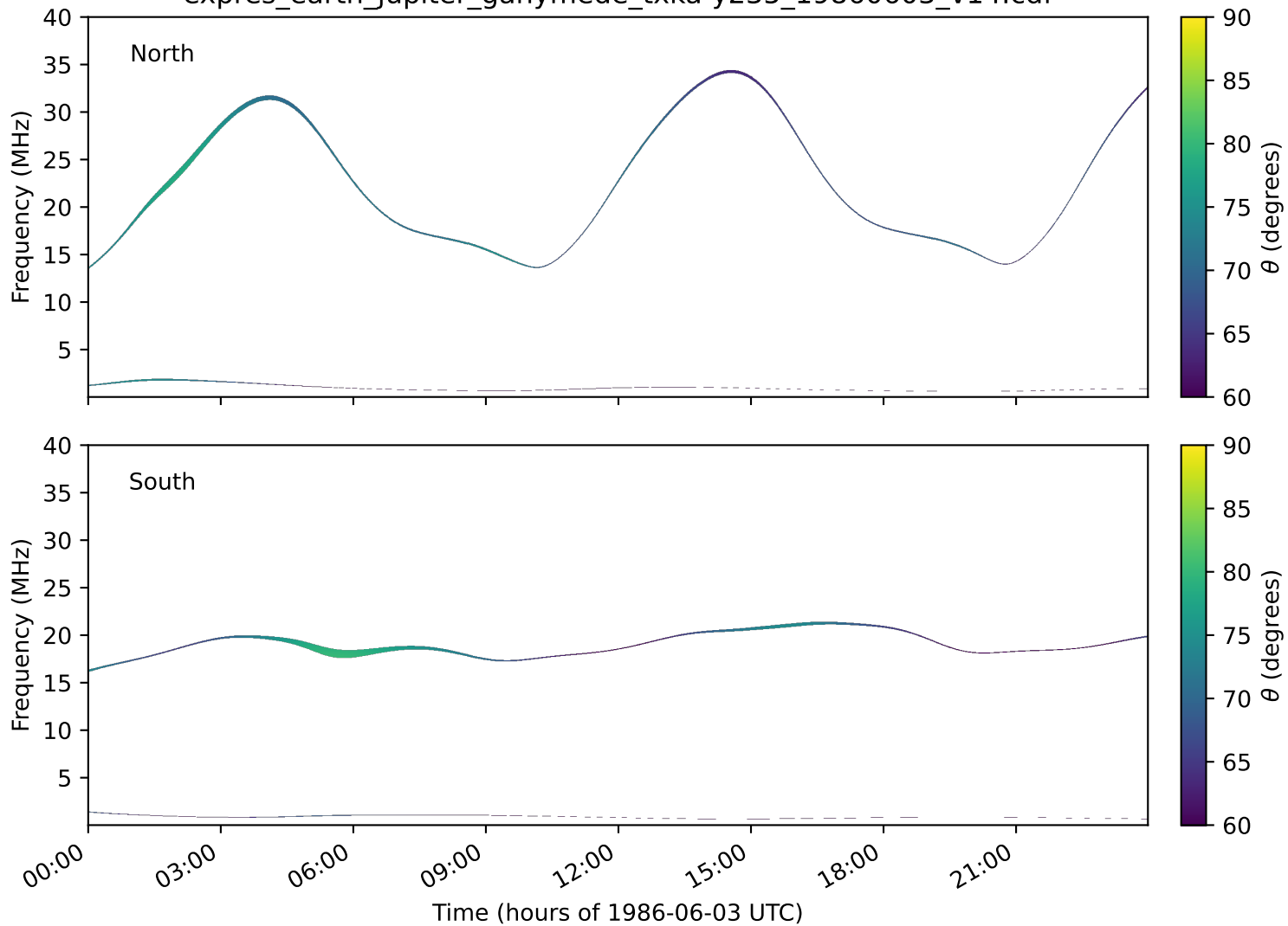
expres_earth_jupiter_ganymede_txka-y235_19860603_v14.cdf
