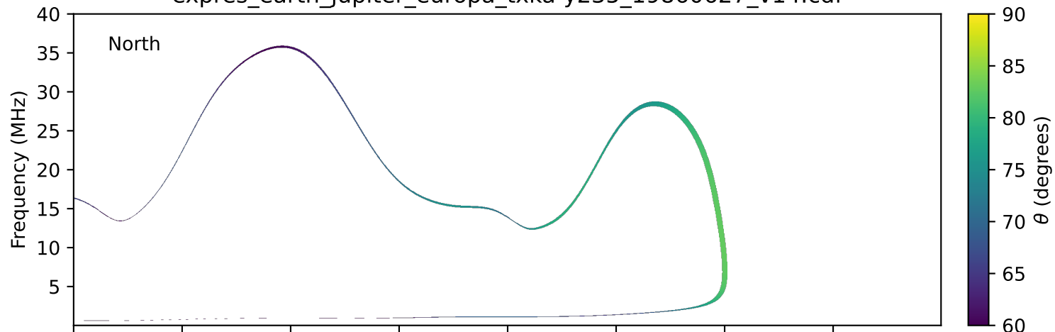
expres_earth_jupiter_europa_txka-y235_19860627_v14.cdf
