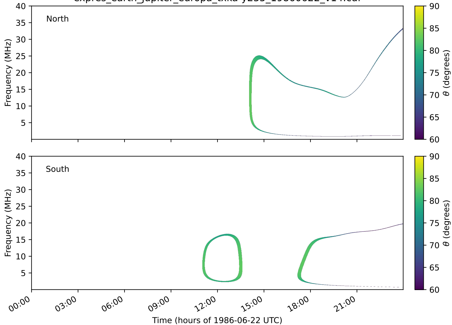
expres_earth_jupiter_europa_txka-y235_19860622_v14.cdf
