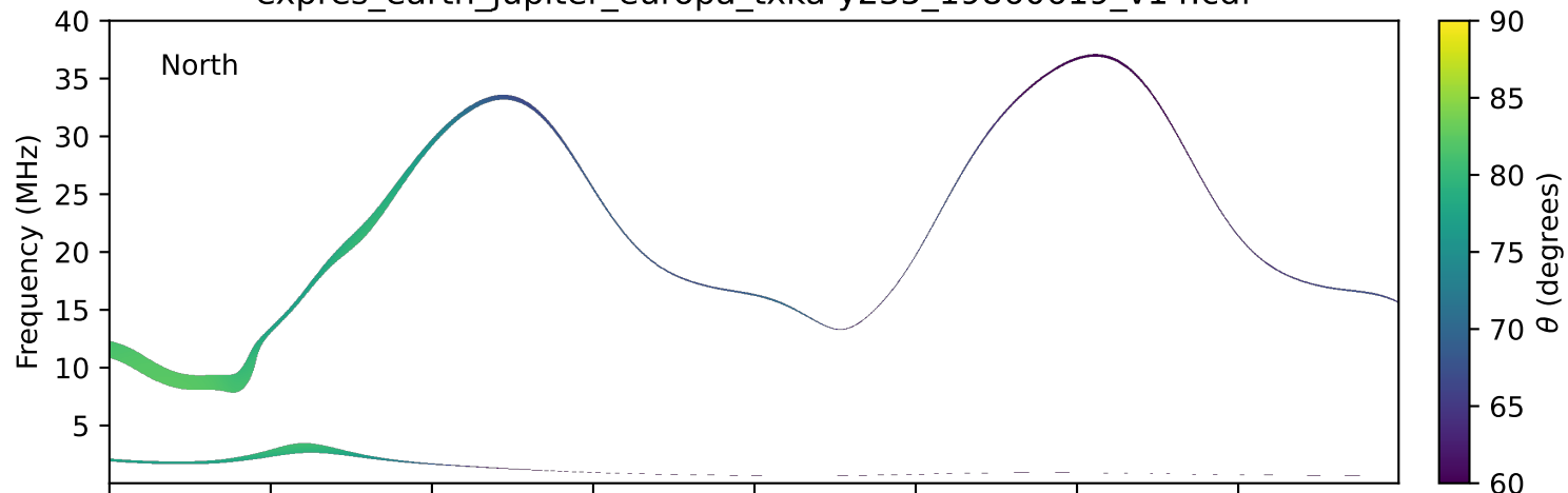
expres_earth_jupiter_europa_txka-y235_19860619_v14.cdf
