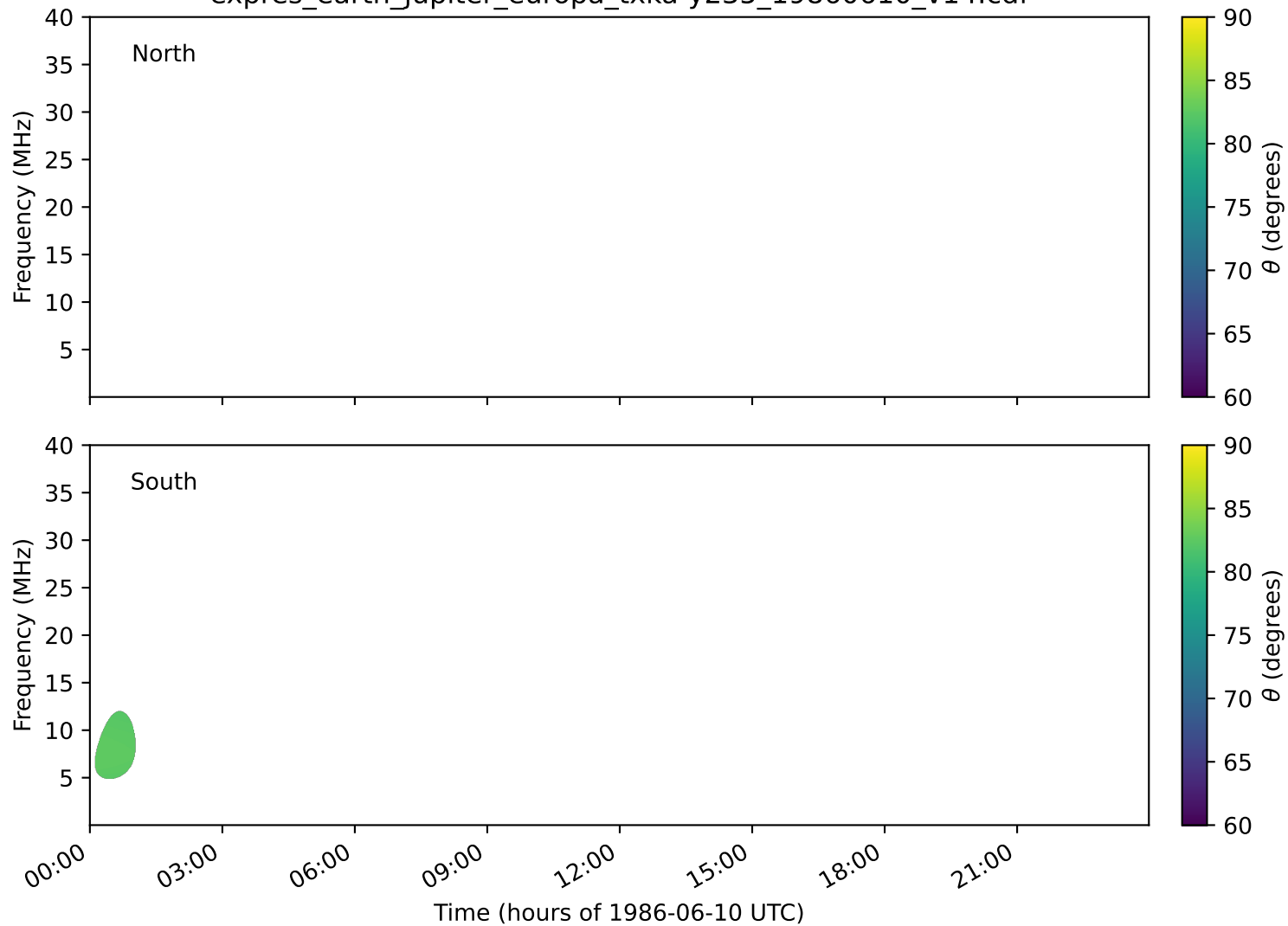
expres_earth_jupiter_europa_txka-y235_19860610_v14.cdf
