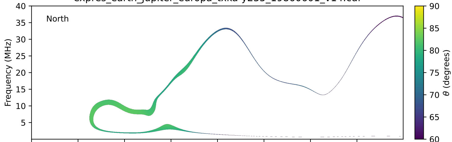
expres_earth_jupiter_europa_txka-y235_19860601_v14.cdf
