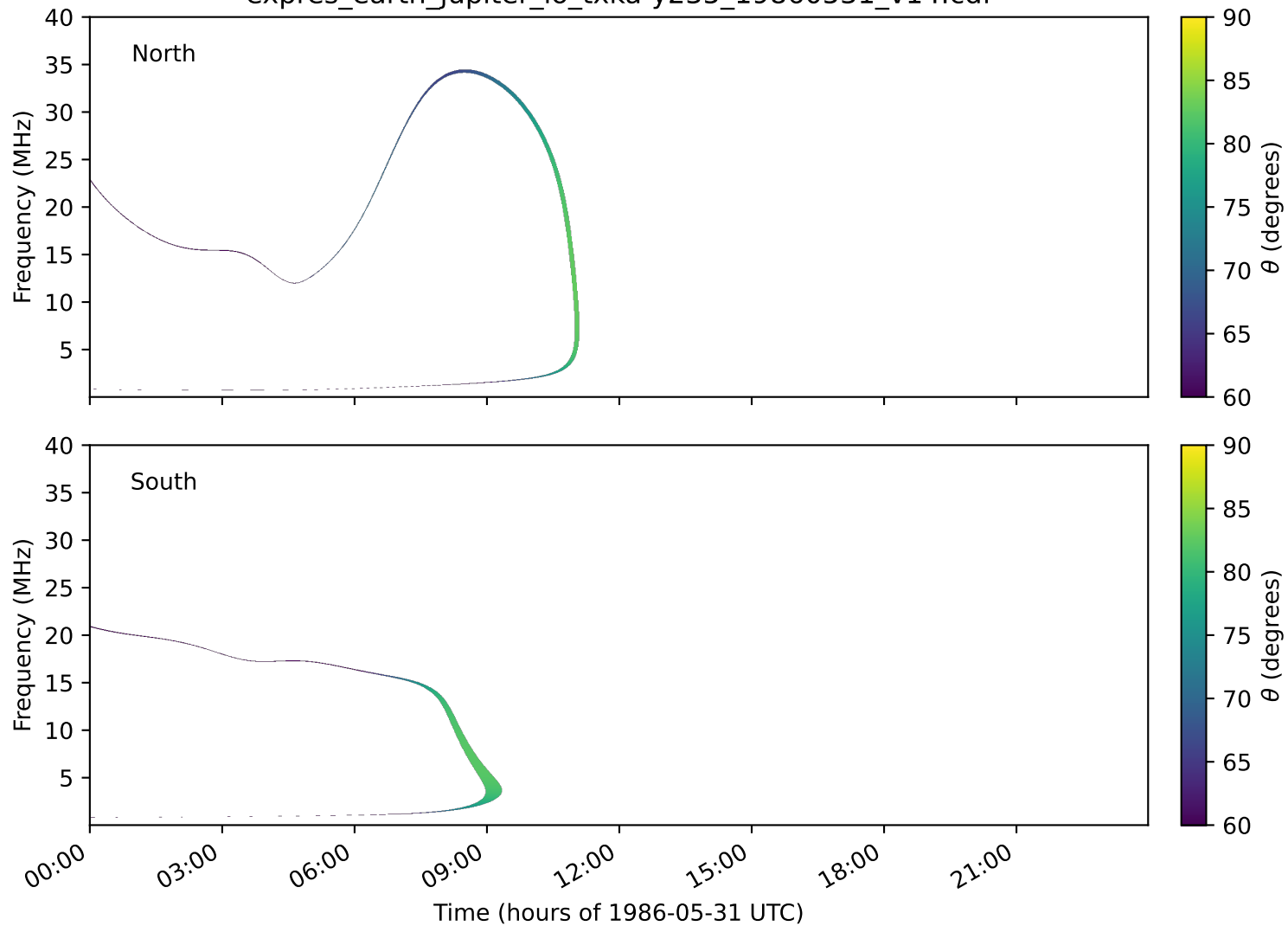
expres_earth_jupiter_io_txka-y235_19860531_v14.cdf
