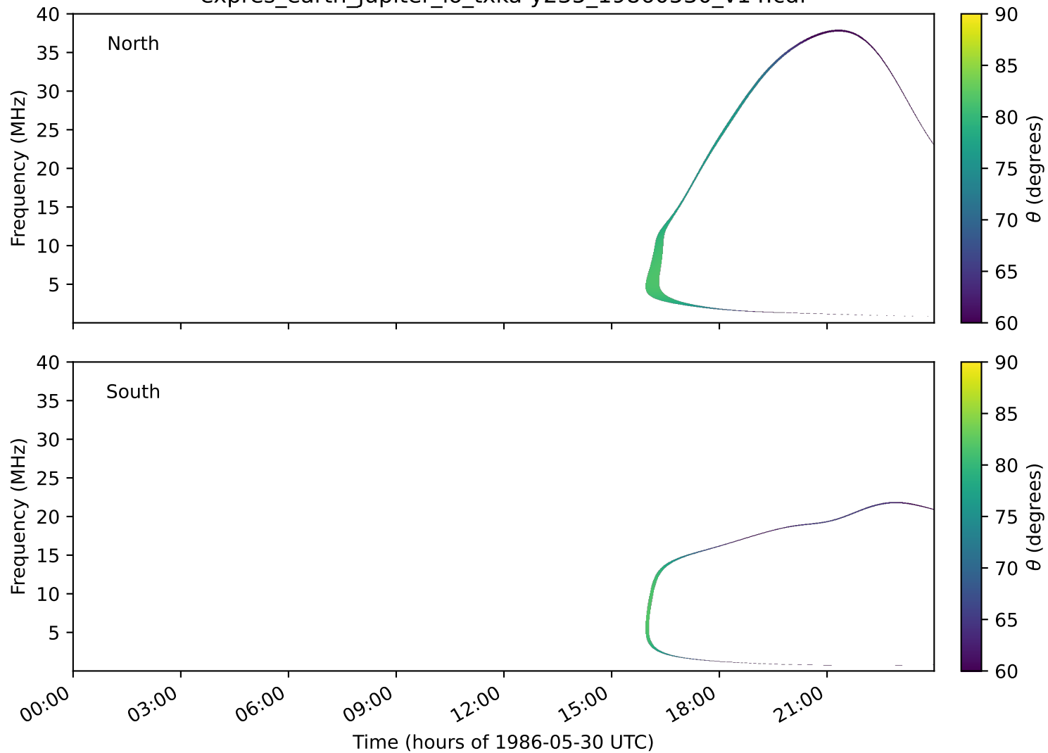
expres_earth_jupiter_io_txka-y235_19860530_v14.cdf
