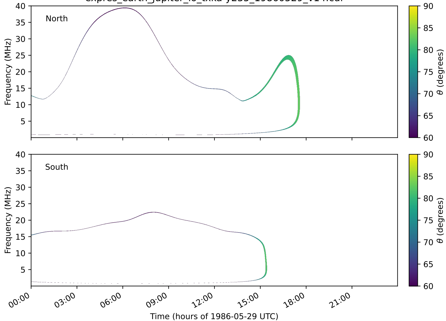
expres_earth_jupiter_io_txka-y235_19860529_v14.cdf
