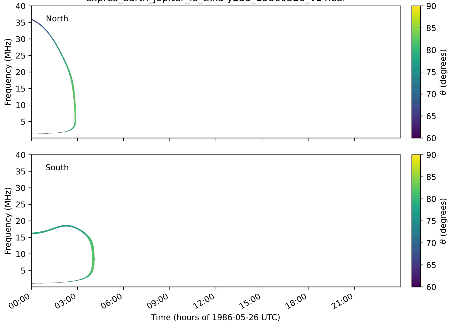
expres_earth_jupiter_io_txka-y235_19860526_v14.cdf
