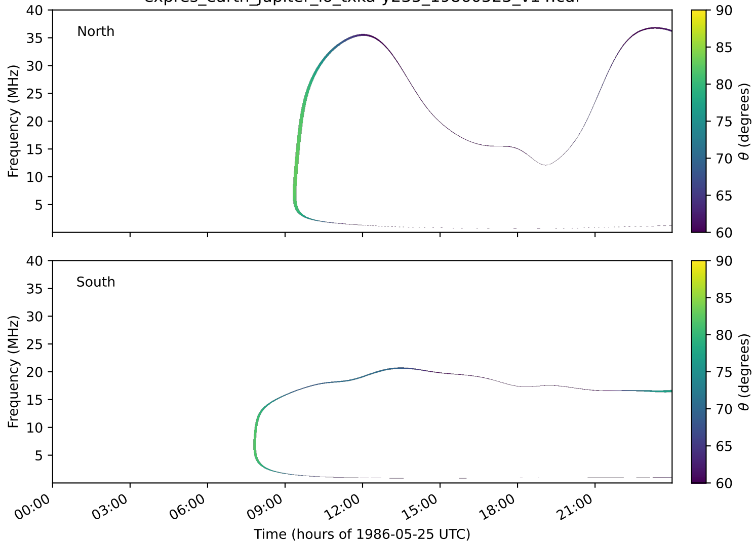
expres_earth_jupiter_io_txka-y235_19860525_v14.cdf
