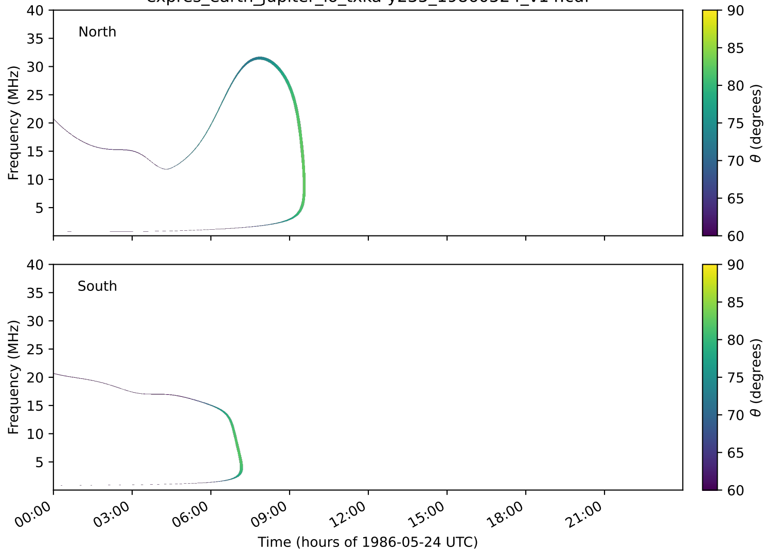
expres_earth_jupiter_io_txka-y235_19860524_v14.cdf
