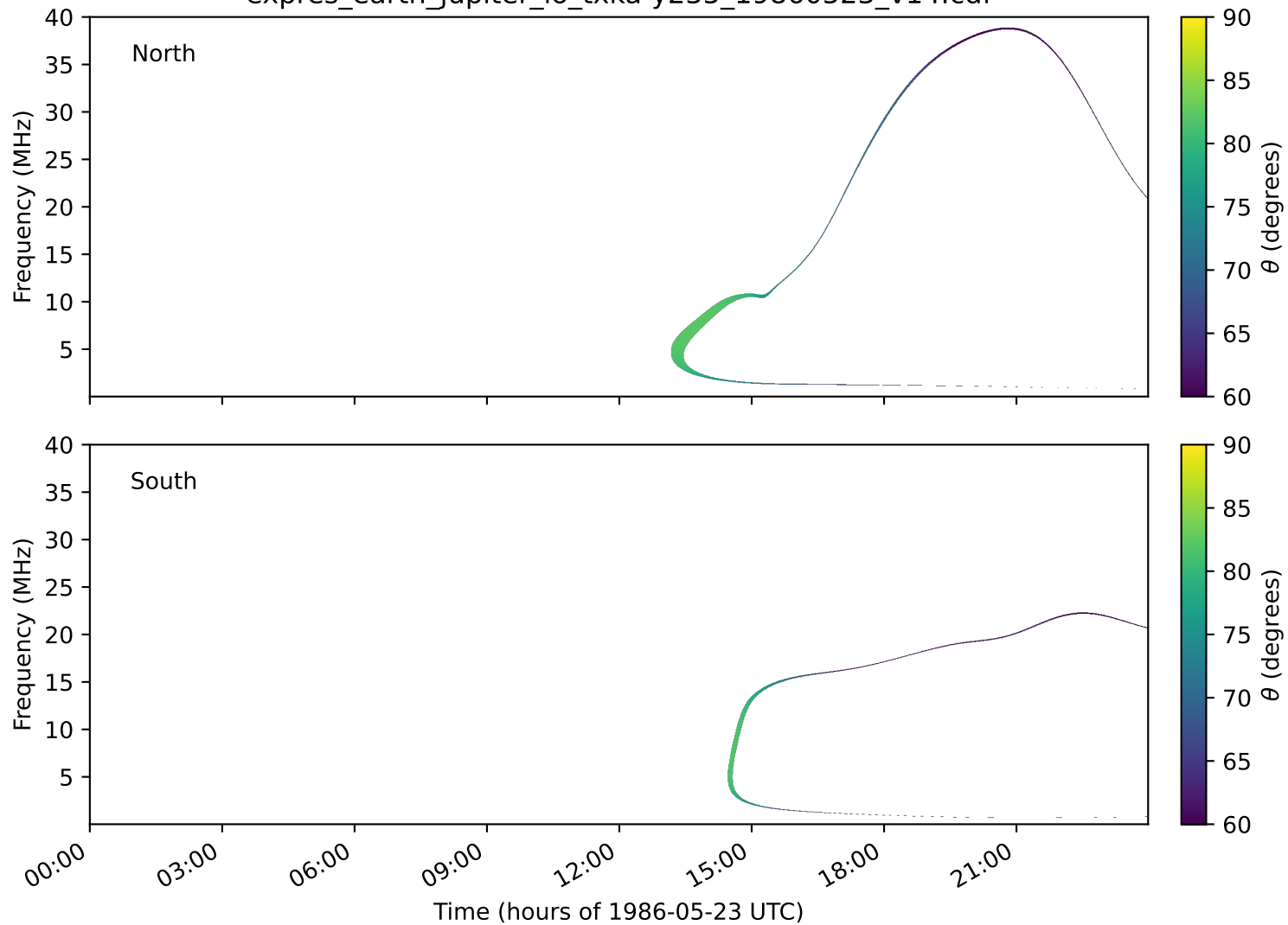
expres_earth_jupiter_io_txka-y235_19860523_v14.cdf
