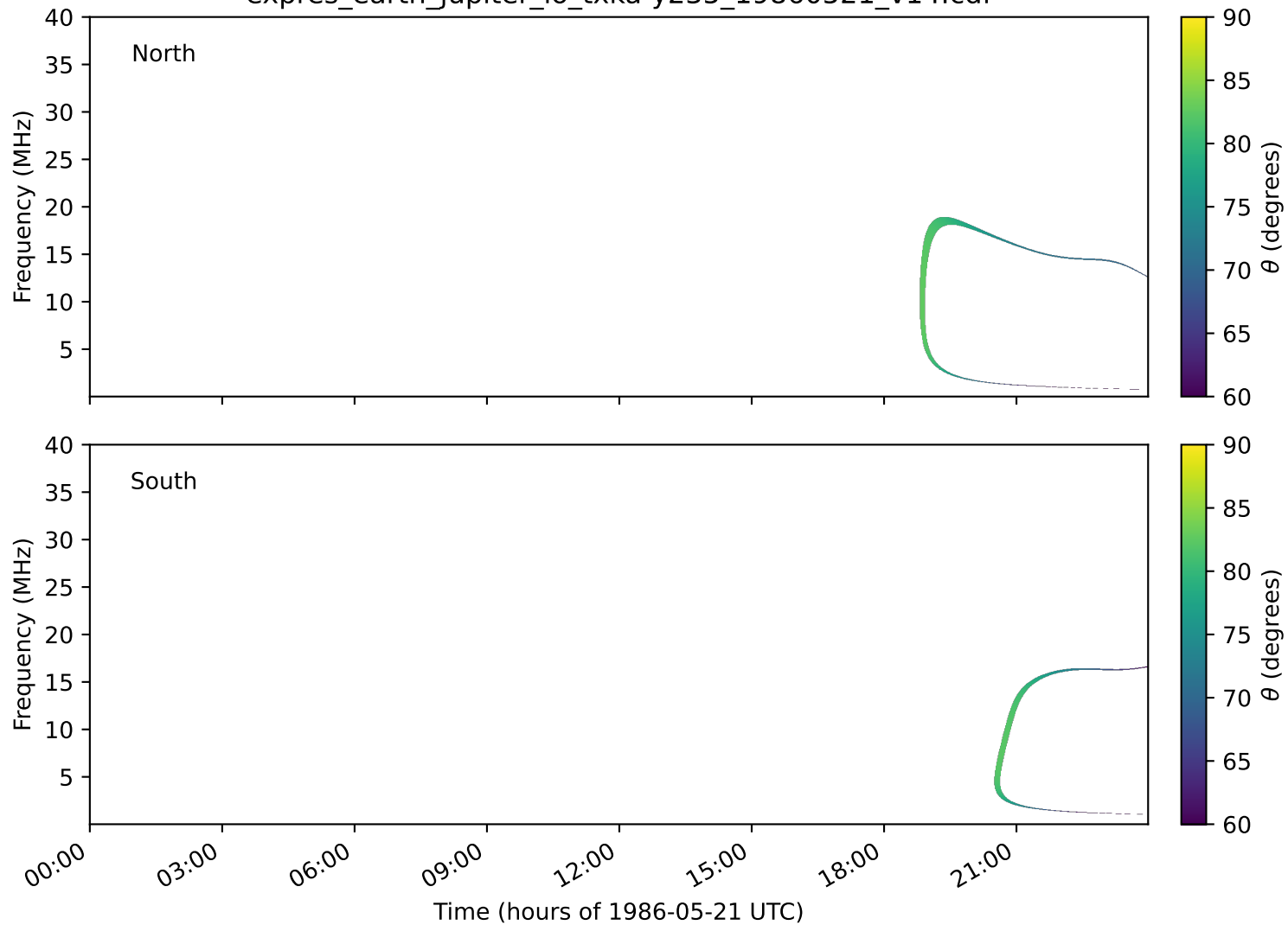
expres_earth_jupiter_io_txka-y235_19860521_v14.cdf
