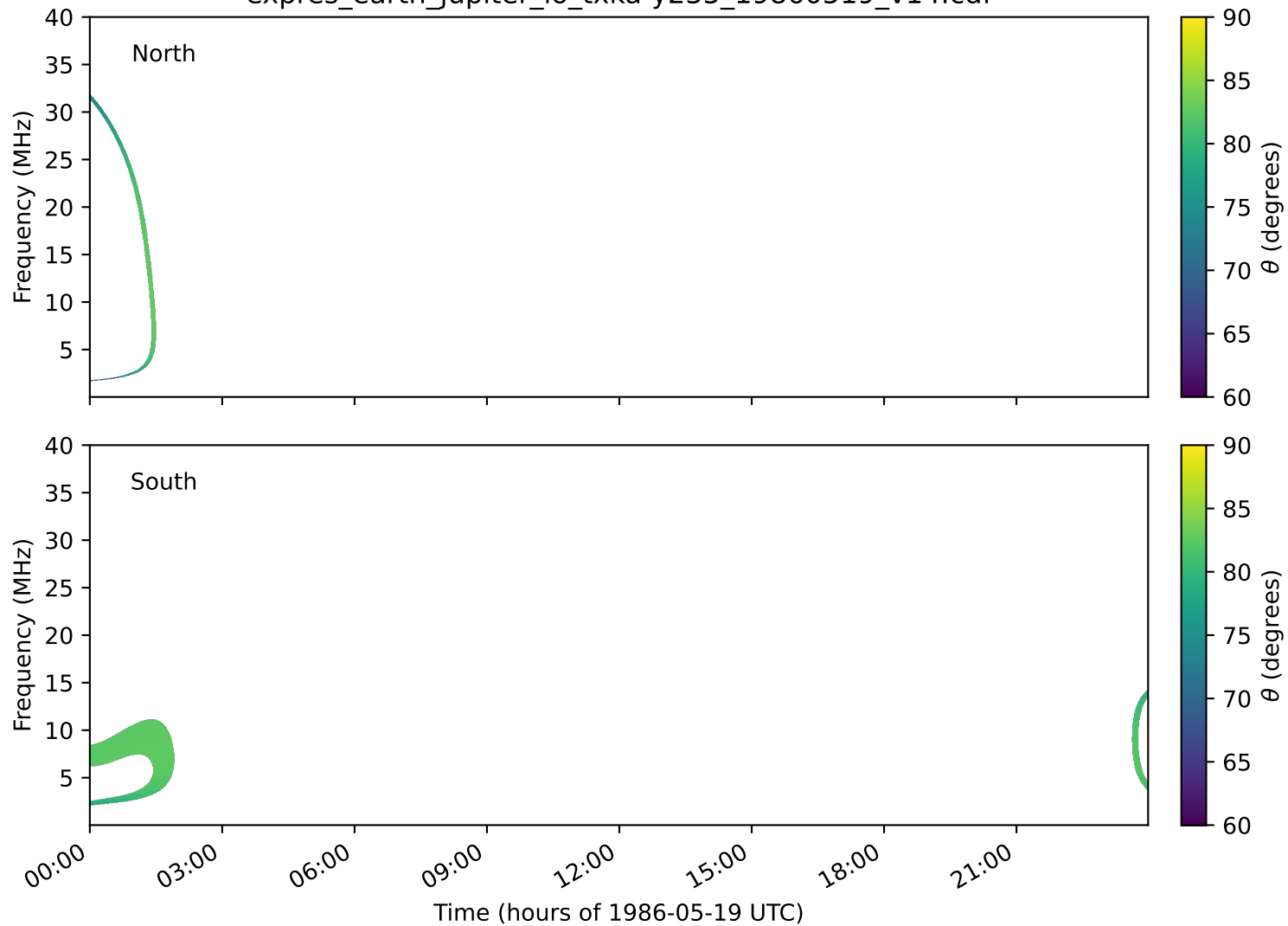
expres_earth_jupiter_io_txka-y235_19860519_v14.cdf
