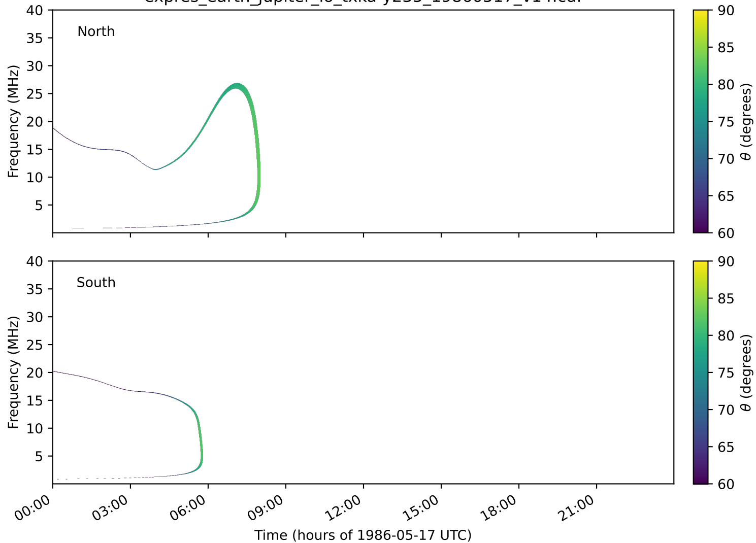
expres_earth_jupiter_io_txka-y235_19860517_v14.cdf
