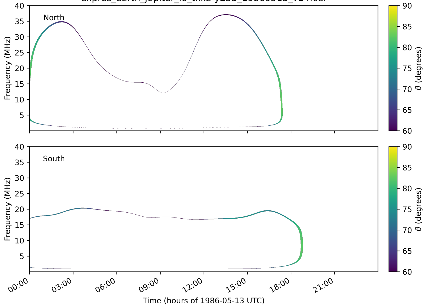
expres_earth_jupiter_io_txka-y235_19860513_v14.cdf
