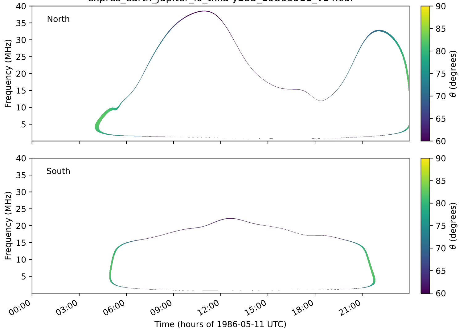
expres_earth_jupiter_io_txka-y235_19860511_v14.cdf
