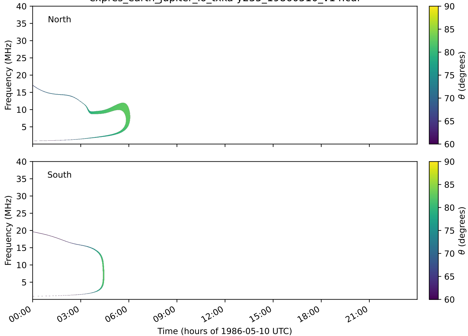
expres_earth_jupiter_io_txka-y235_19860510_v14.cdf
