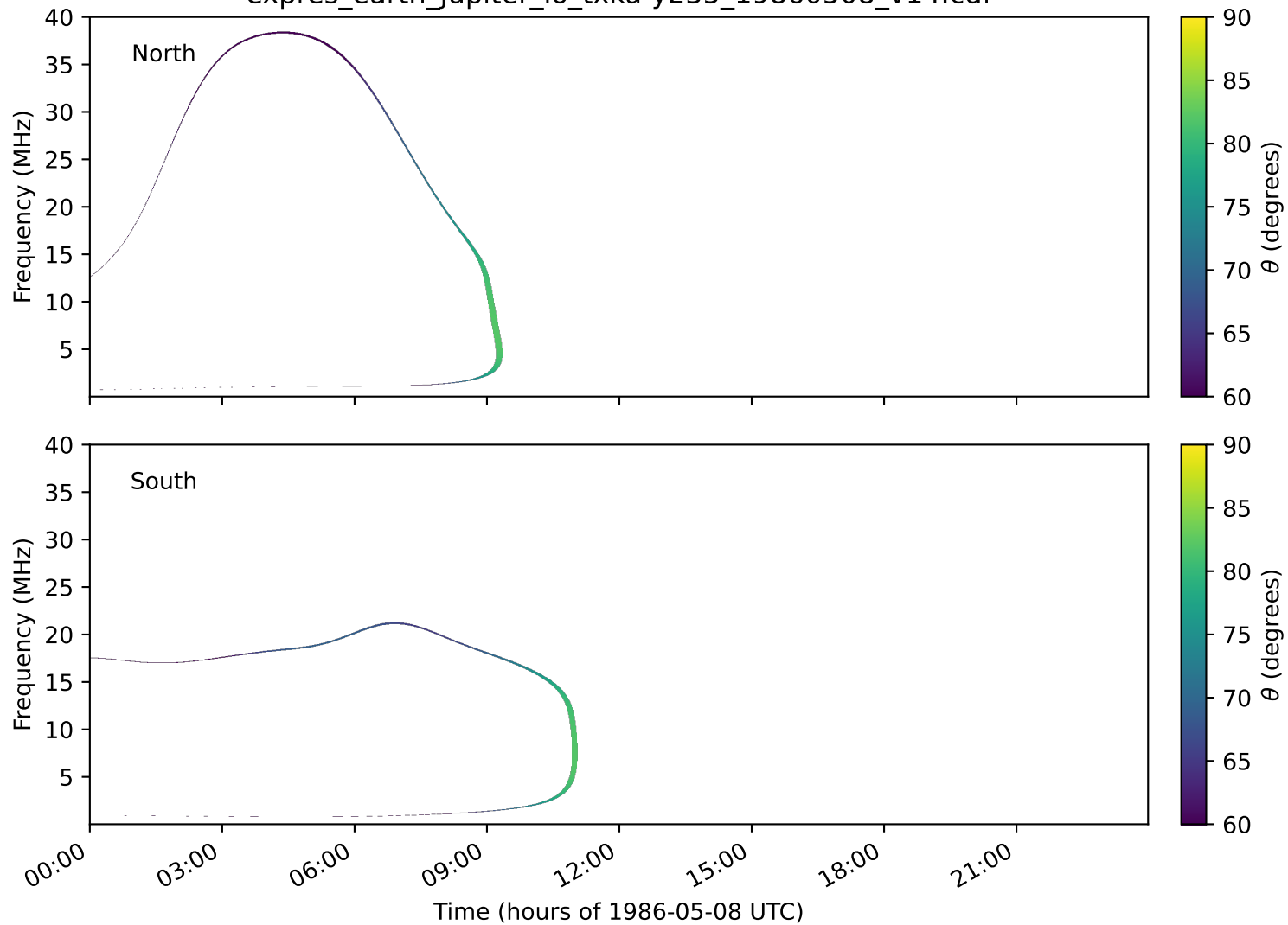
expres_earth_jupiter_io_txka-y235_19860508_v14.cdf
