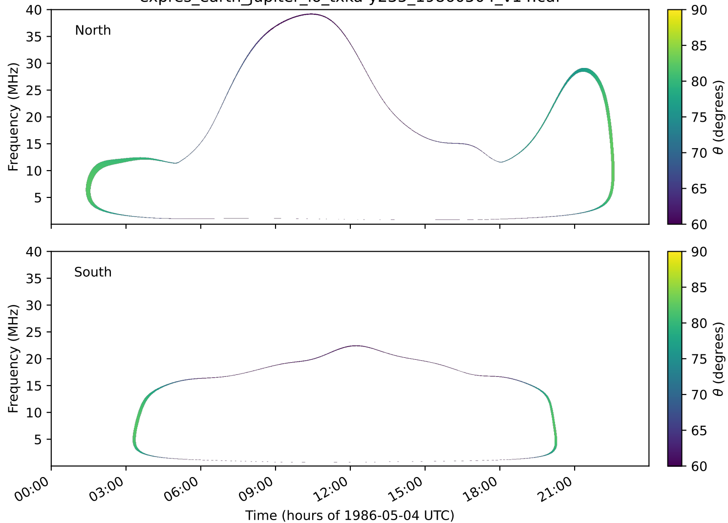
expres_earth_jupiter_io_txka-y235_19860504_v14.cdf
