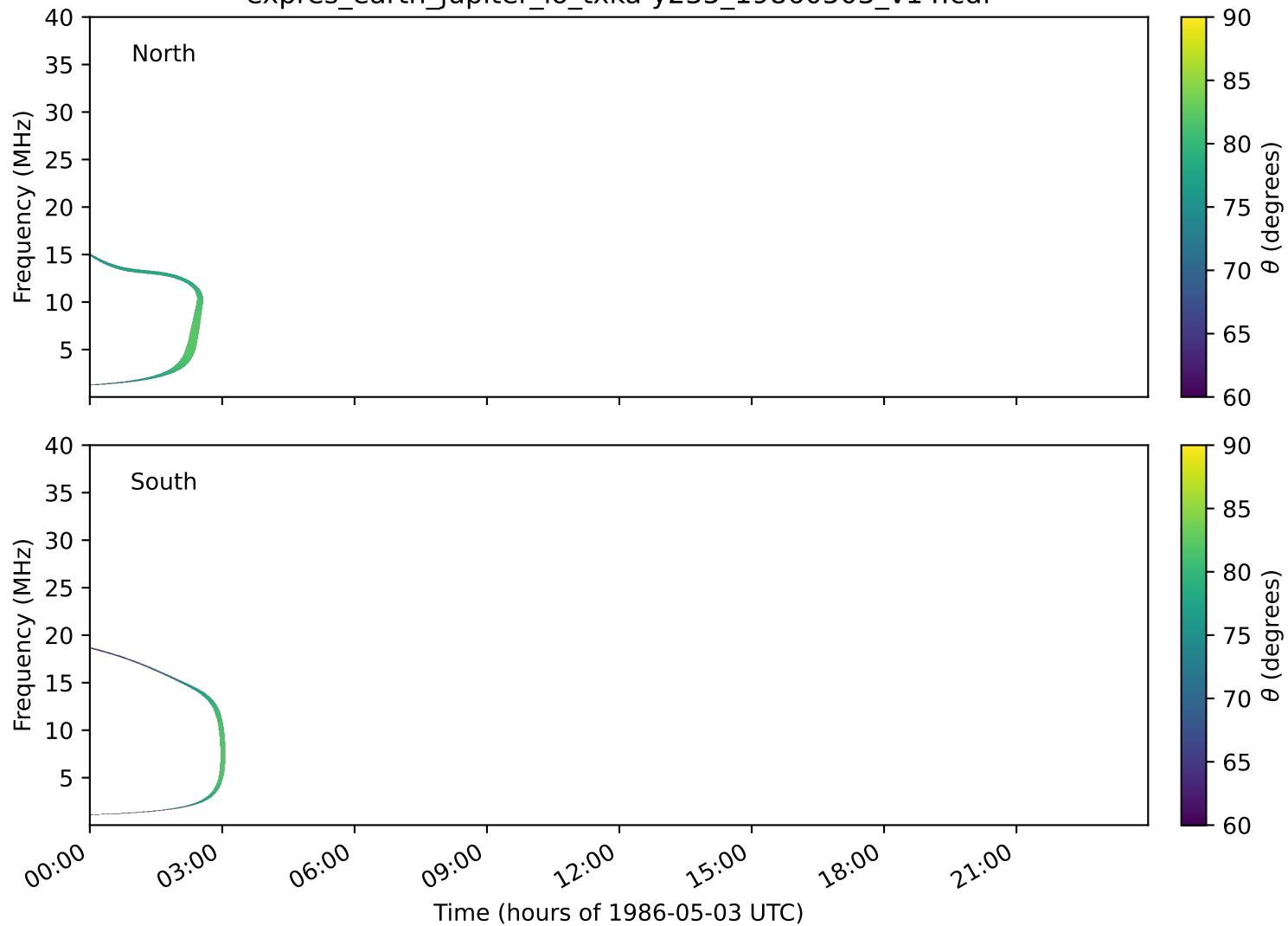
expres_earth_jupiter_io_txka-y235_19860503_v14.cdf
