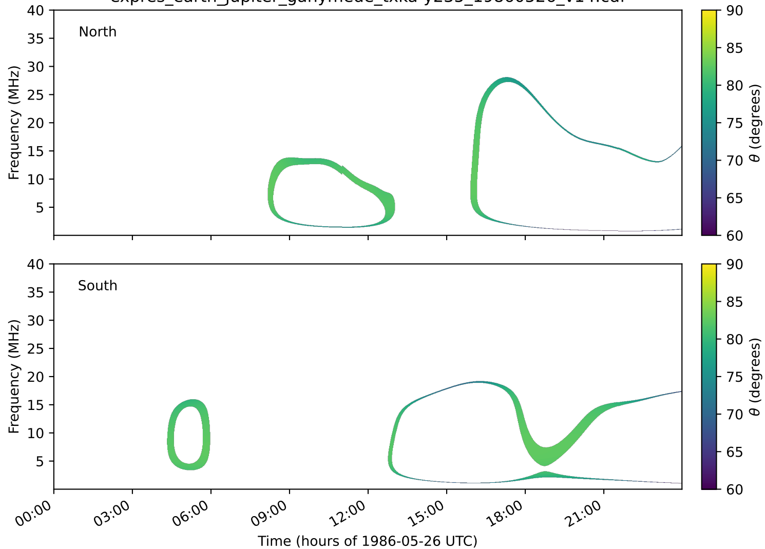
expres_earth_jupiter_ganymede_txka-y235_19860526_v14.cdf
