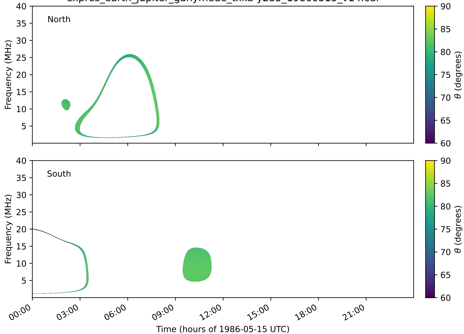
expres_earth_jupiter_ganymede_txka-y235_19860515_v14.cdf
