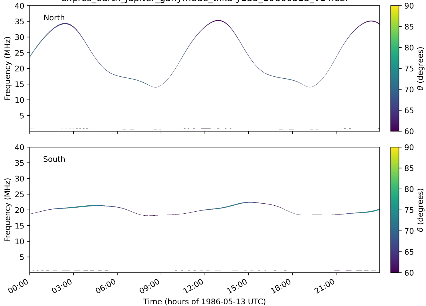
expres_earth_jupiter_ganymede_txka-y235_19860513_v14.cdf
