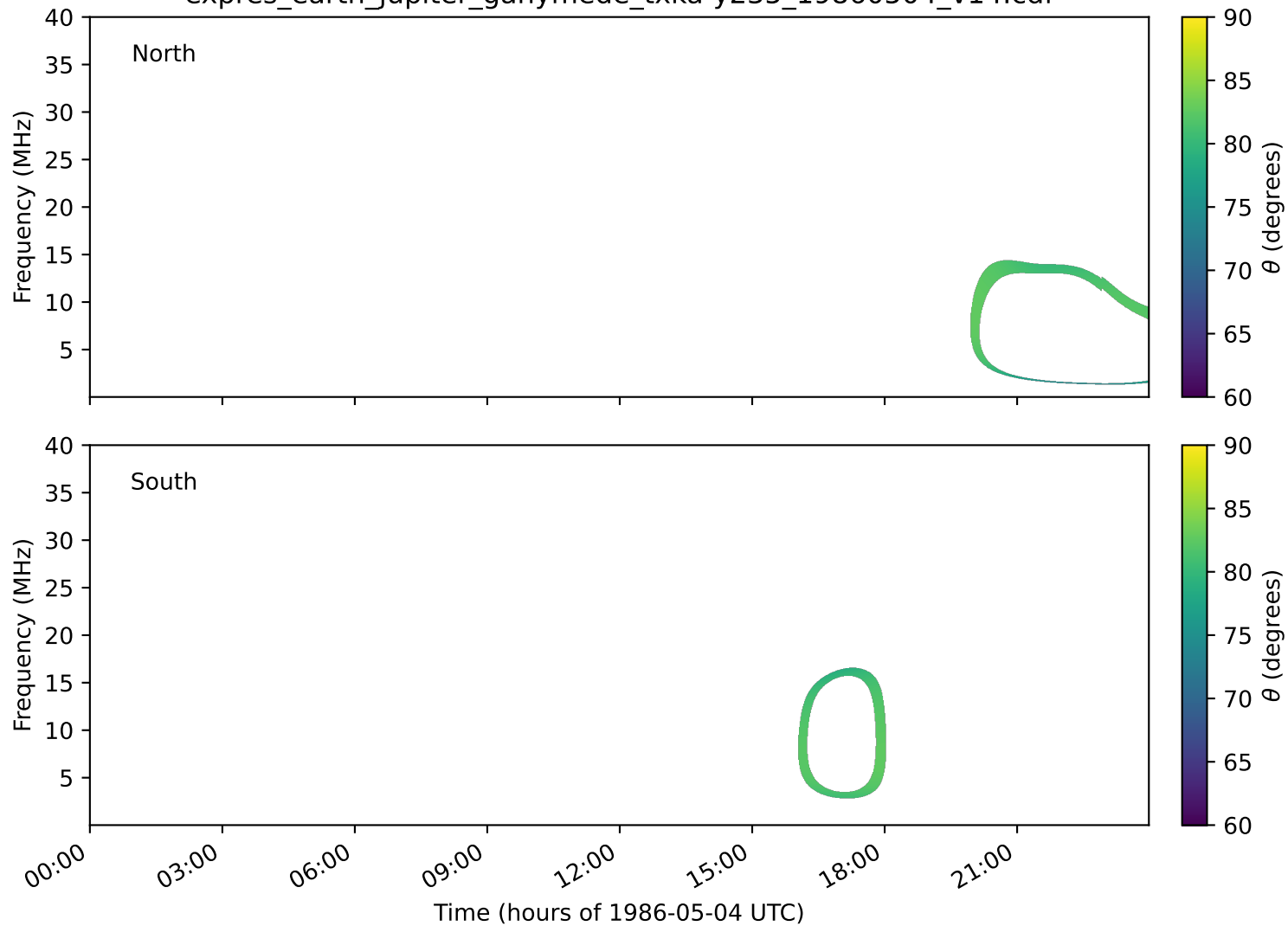
expres_earth_jupiter_ganymede_txka-y235_19860504_v14.cdf
