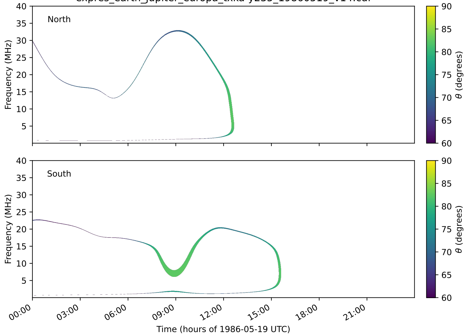
expres_earth_jupiter_europa_txka-y235_19860519_v14.cdf
