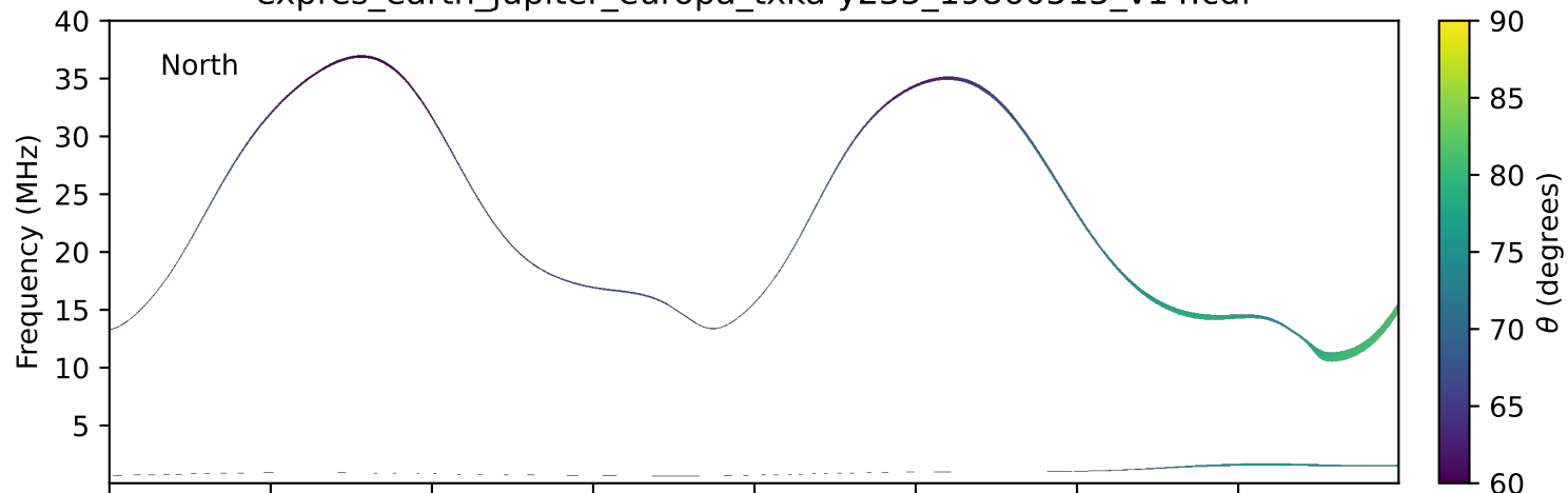
expres_earth_jupiter_europa_txka-y235_19860515_v14.cdf
