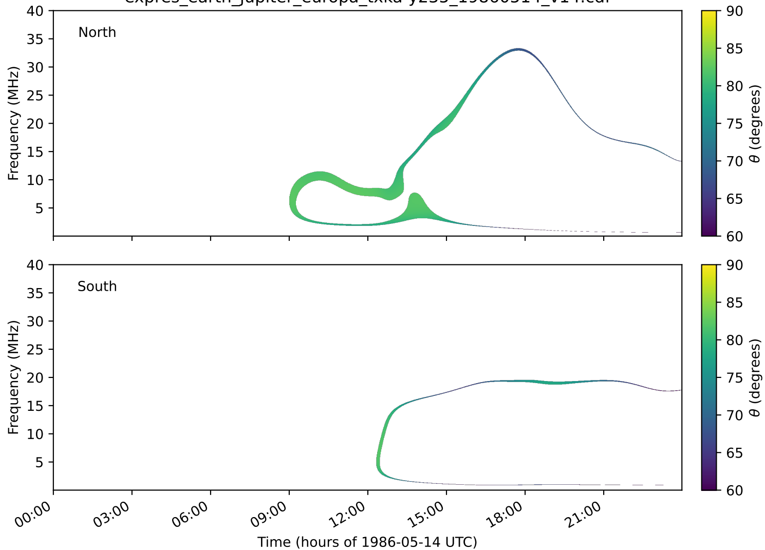
expres_earth_jupiter_europa_txka-y235_19860514_v14.cdf
