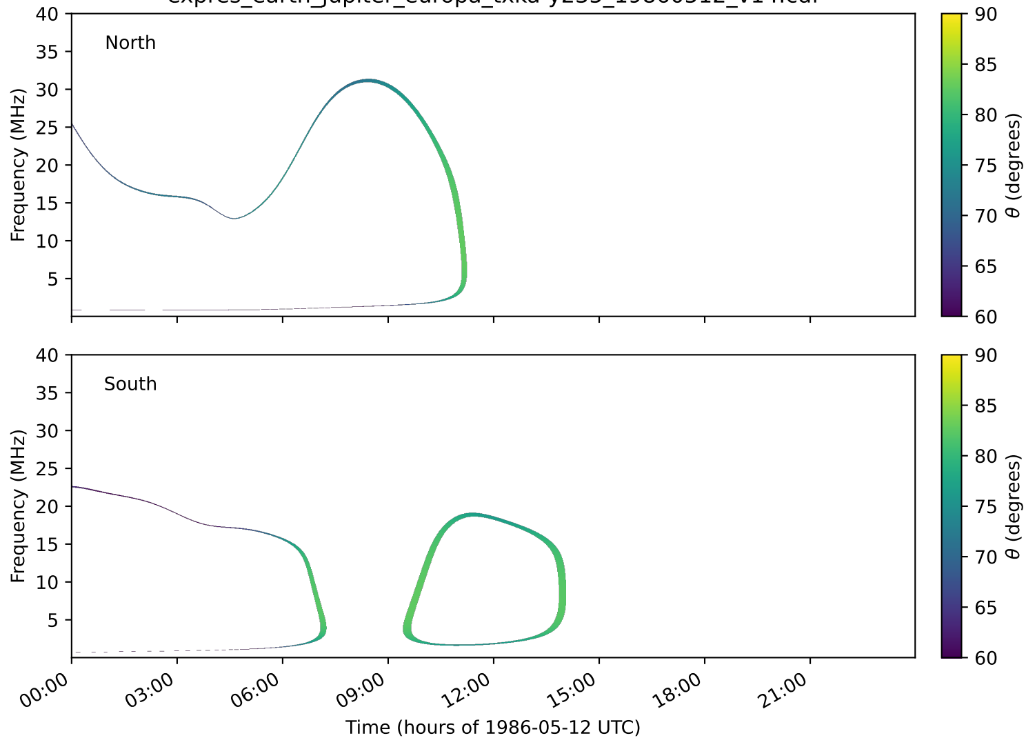
expres_earth_jupiter_europa_txka-y235_19860512_v14.cdf
