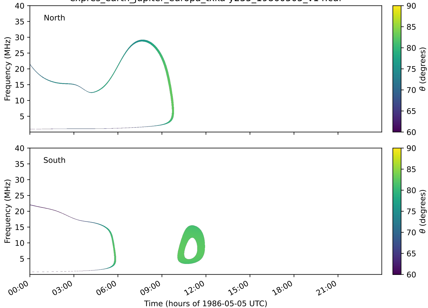
expres_earth_jupiter_europa_txka-y235_19860505_v14.cdf
