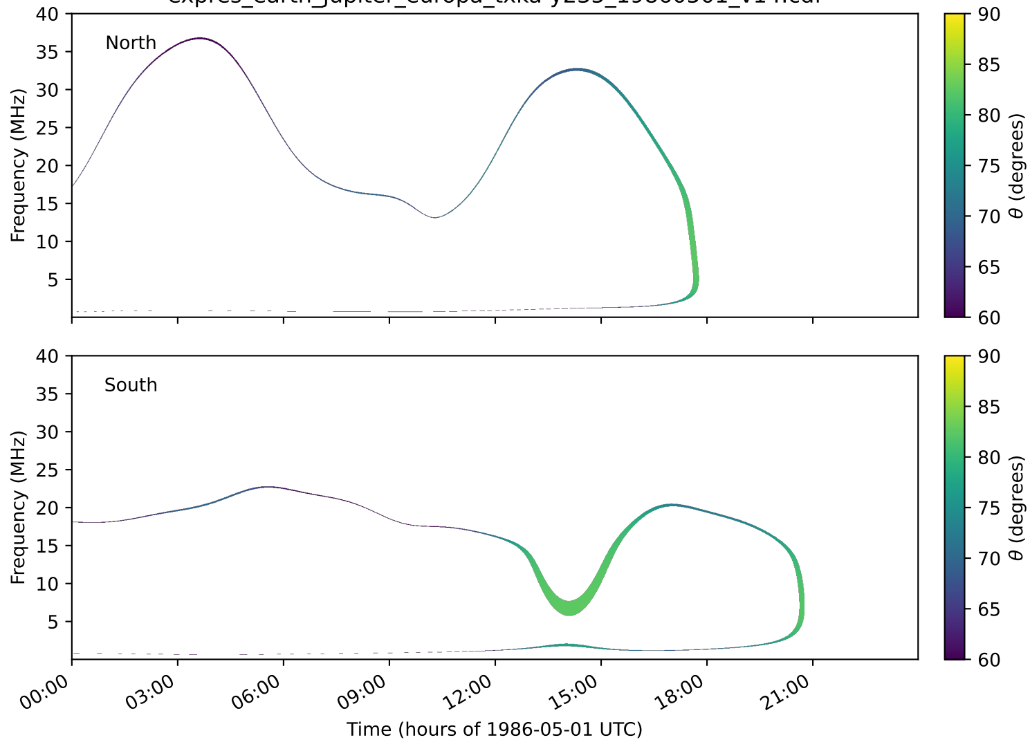
expres_earth_jupiter_europa_txka-y235_19860501_v14.cdf
