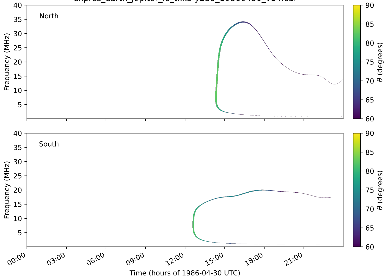
expres_earth_jupiter_io_txka-y235_19860430_v14.cdf
