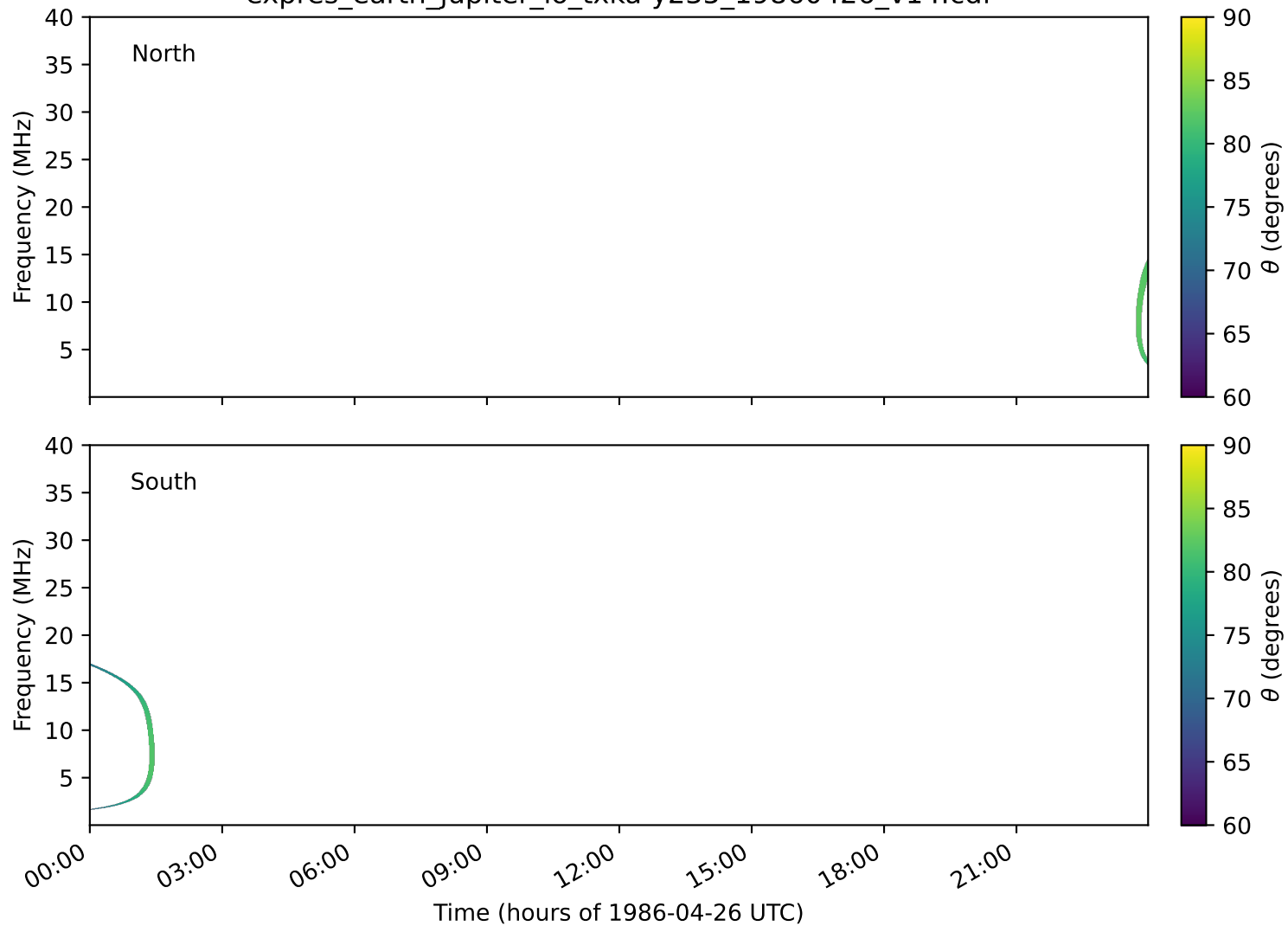
expres_earth_jupiter_io_txka-y235_19860426_v14.cdf
