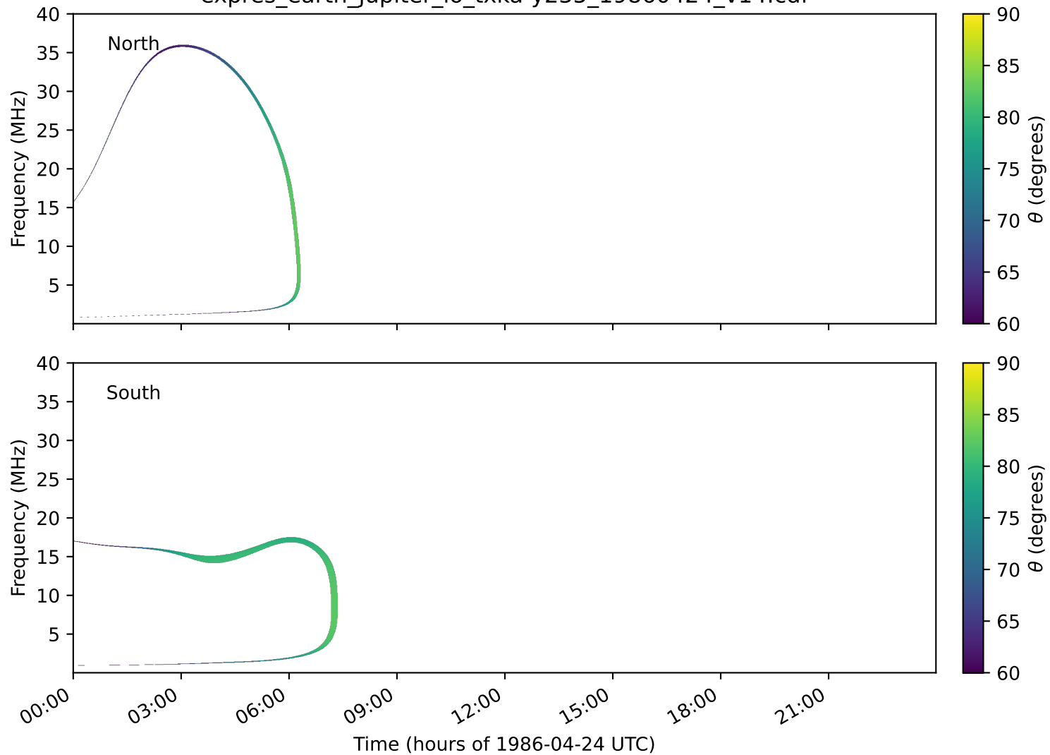
expres_earth_jupiter_io_txka-y235_19860424_v14.cdf
