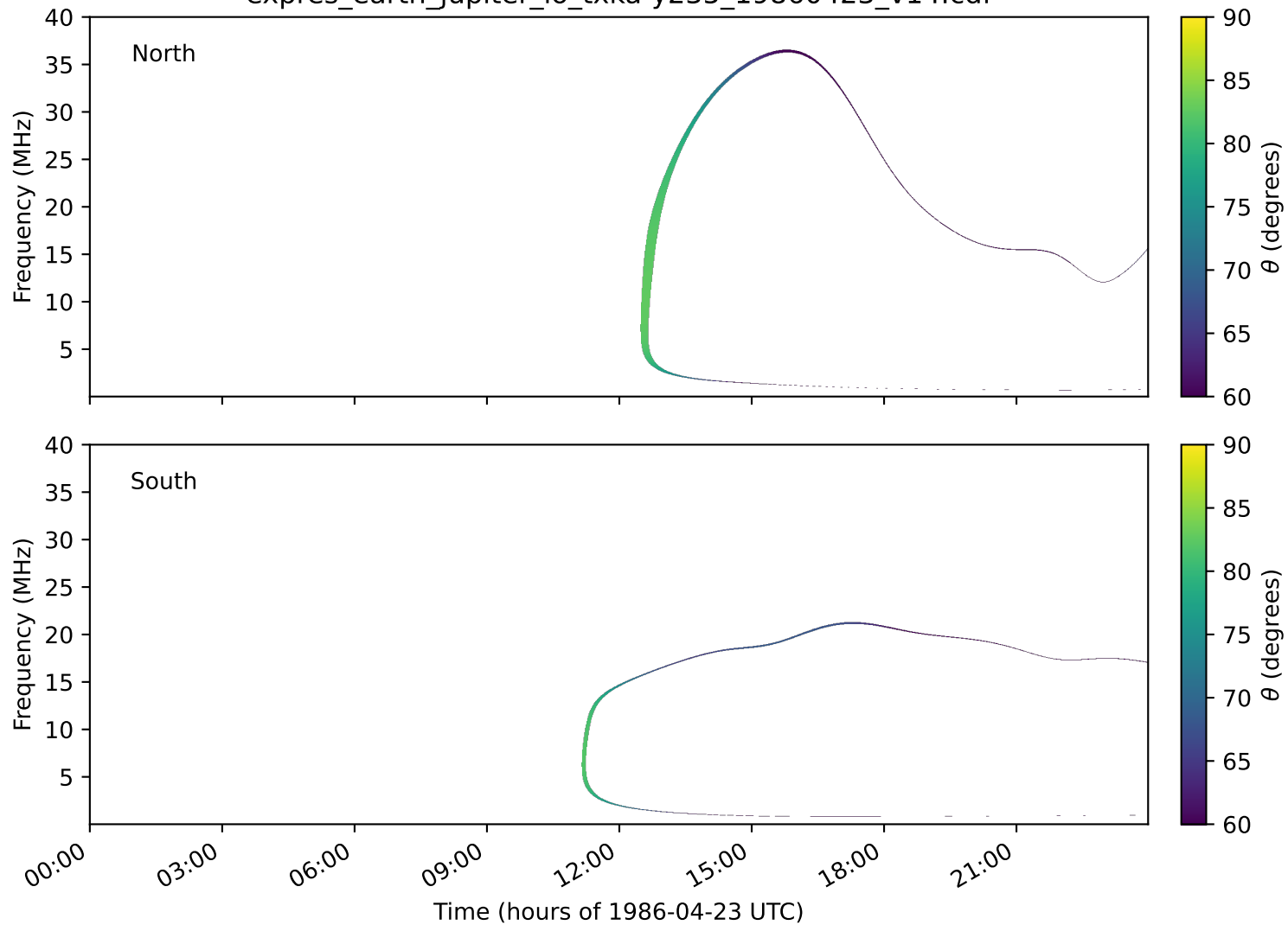
expres_earth_jupiter_io_txka-y235_19860423_v14.cdf
