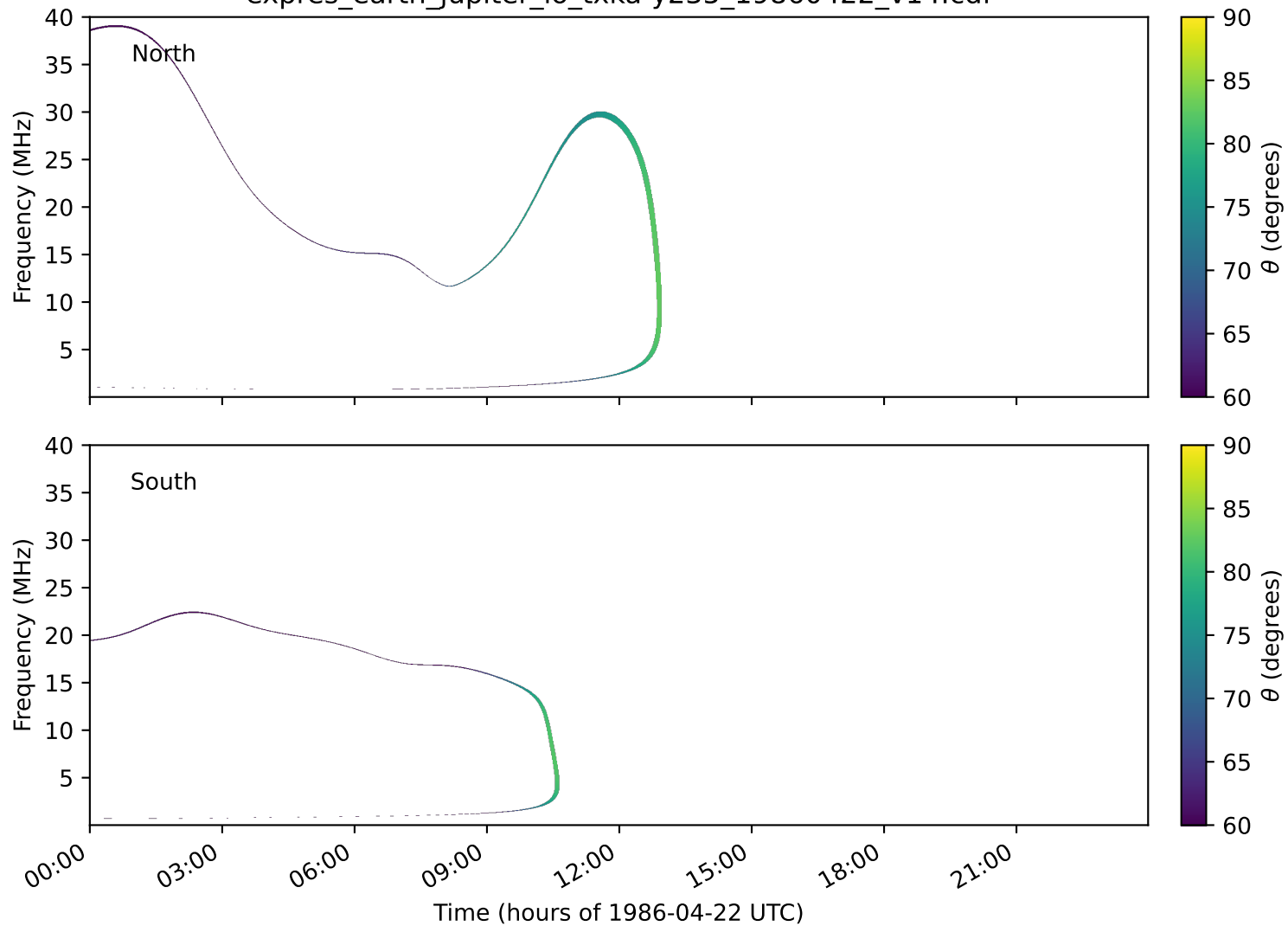
expres_earth_jupiter_io_txka-y235_19860422_v14.cdf
