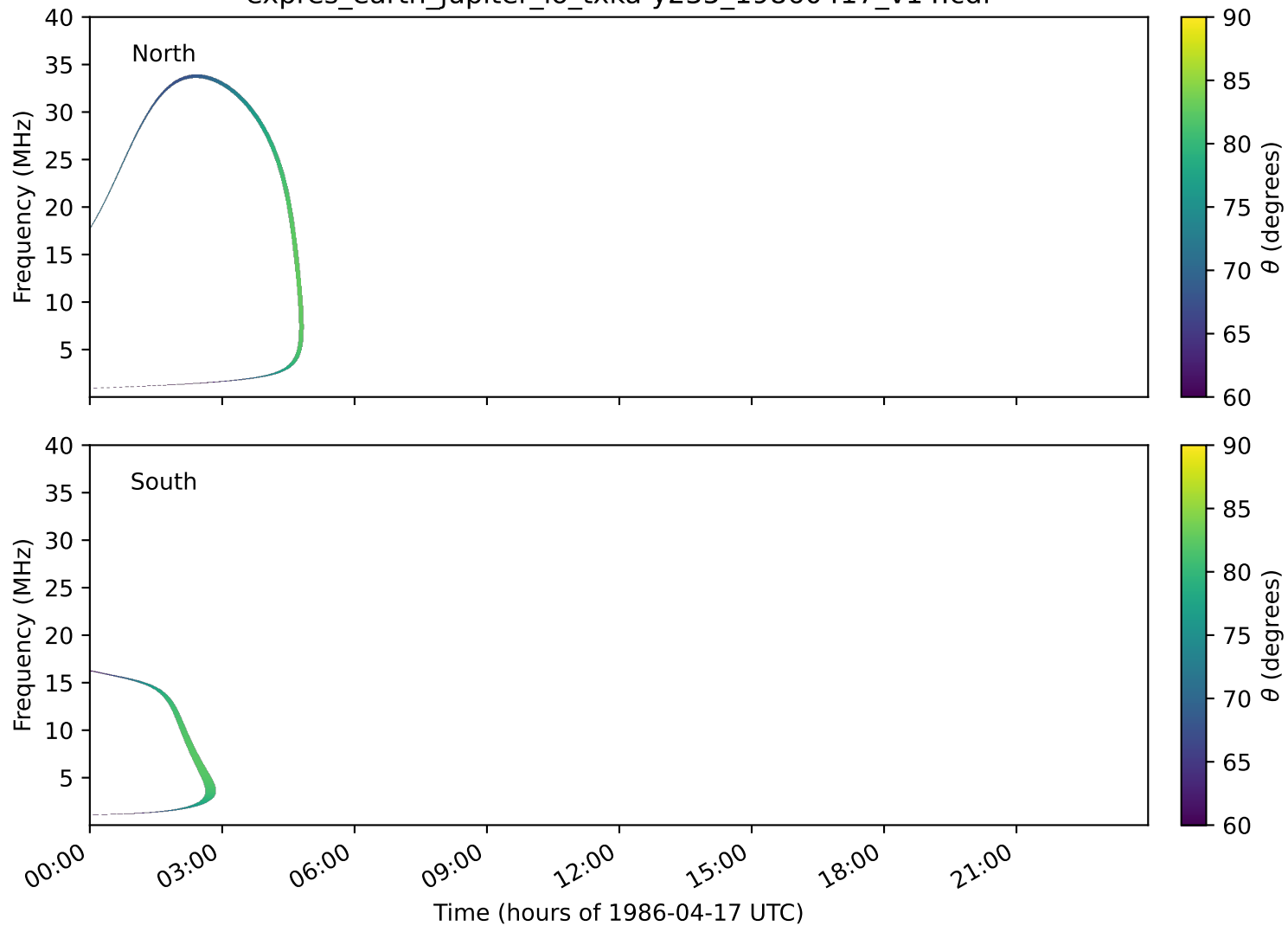
expres_earth_jupiter_io_txka-y235_19860417_v14.cdf
