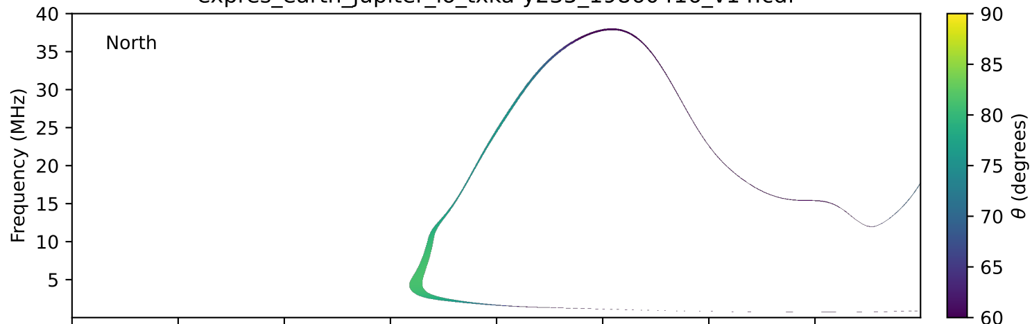
expres_earth_jupiter_io_txka-y235_19860416_v14.cdf
