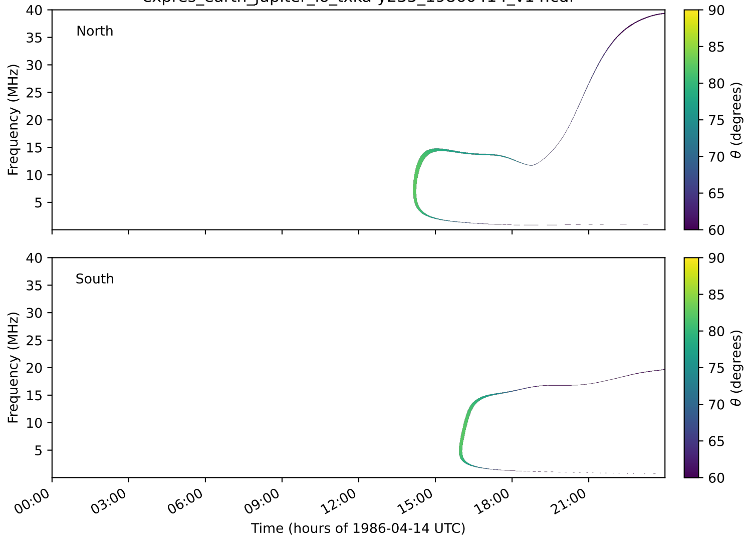
expres_earth_jupiter_io_txka-y235_19860414_v14.cdf
