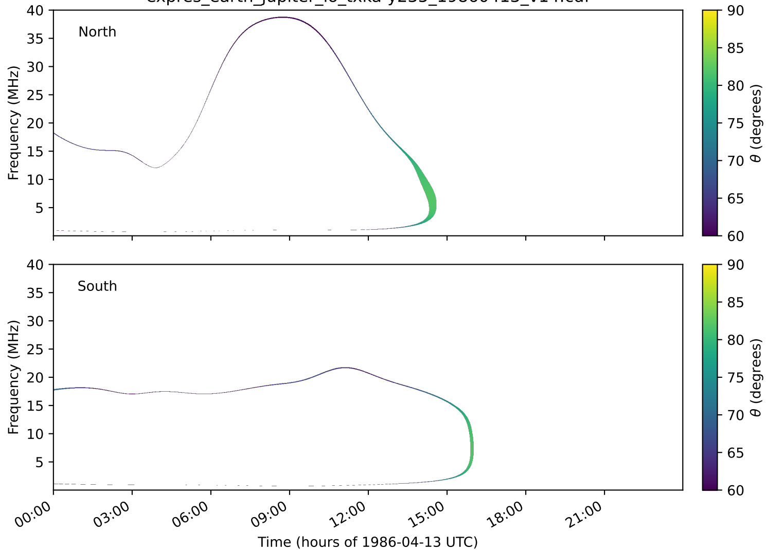
expres_earth_jupiter_io_txka-y235_19860413_v14.cdf
